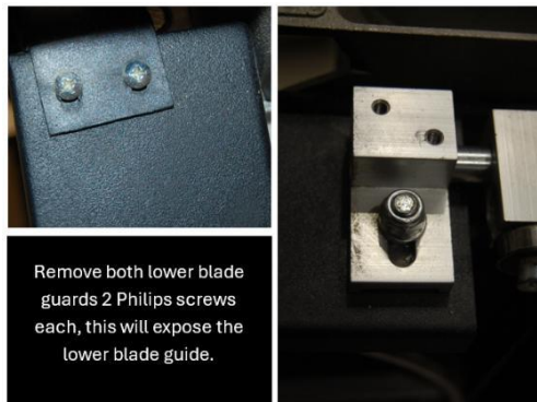
Figure 9: Lower blade guards.
