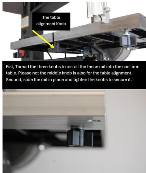
Figure 6: Installing the Rail and Fence.
