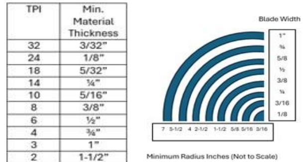
Figure 12: Cut Radius and Material thickness
