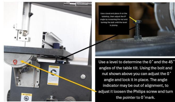
Figure 25: Table tilt adjustments.
