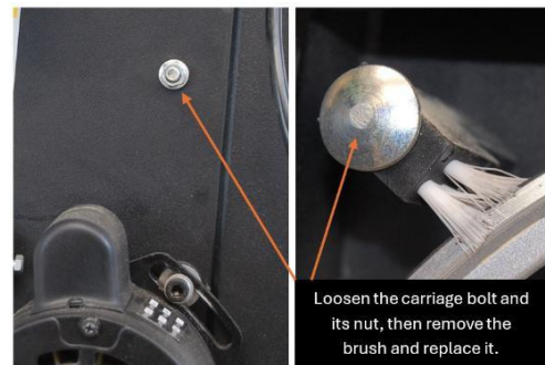
Figure 21: Adjusting/ Replacing the lower wheel brush.
