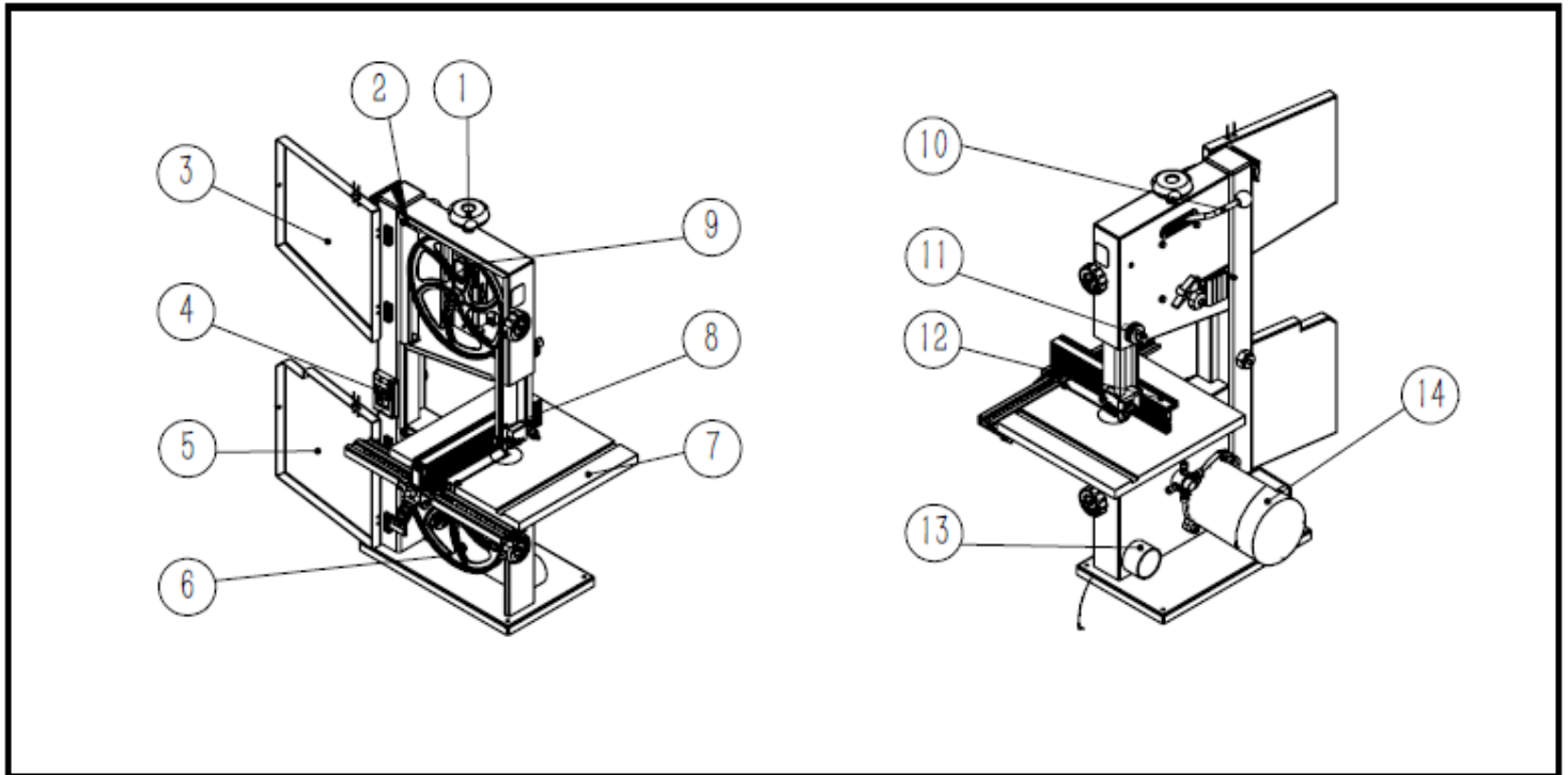
Figure 1: Machine Identification.
