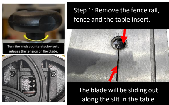
Figure 13: removing the rail and table insert.
