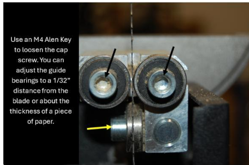
Figure 10: Adjusting the lower blade guide.
