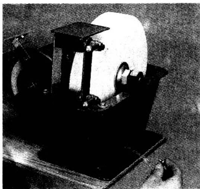
SCREW- Remove the screw to drain the water. (FIG 10 )
