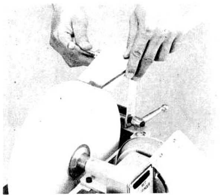
Sliding angle jig facilitates sharpening double-angle cutting tools.
